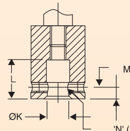
DETAIL "D1"
