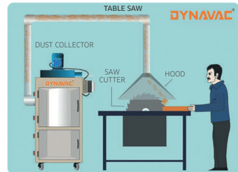
Dust extraction from sawing operation with canopy hood
